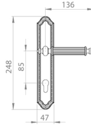
YALE TİP / CYLINDRICAL TYPE
